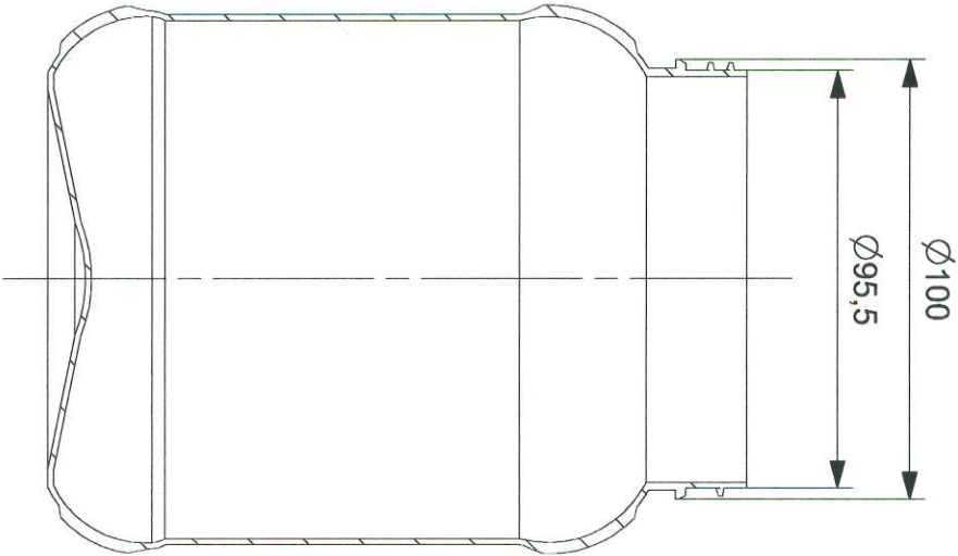
SECTION C-C
