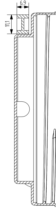
SECTION B-B
