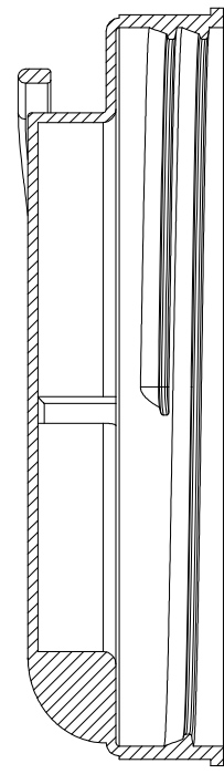
SECTION B-B
