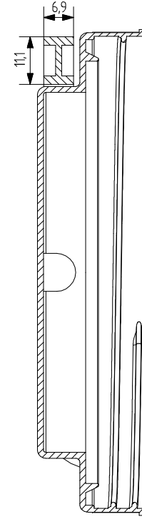
SECTION B-B
